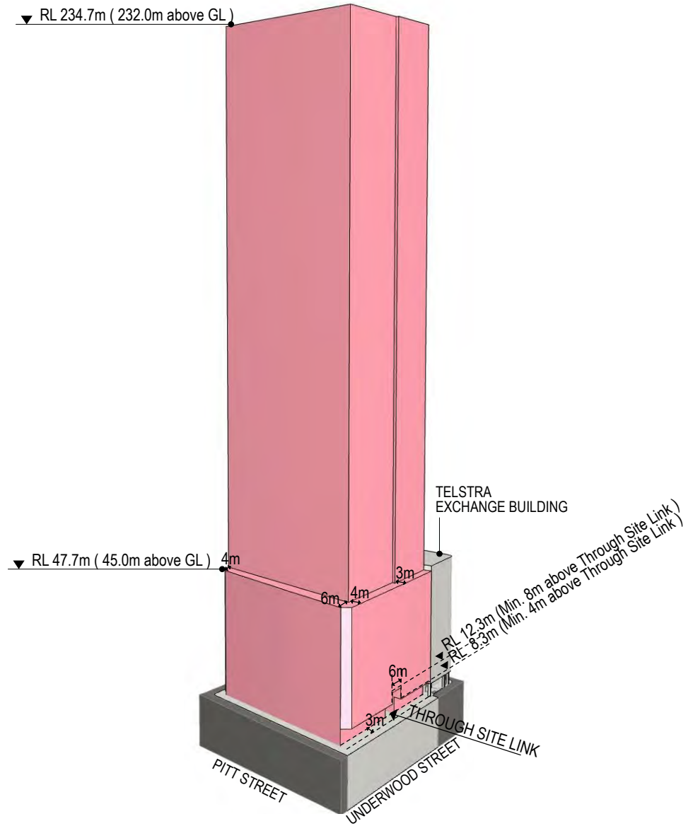
Figure 6.18a North-west View Development Control Envelope – 55 Pitt Street
